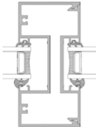
Mullion Detail
