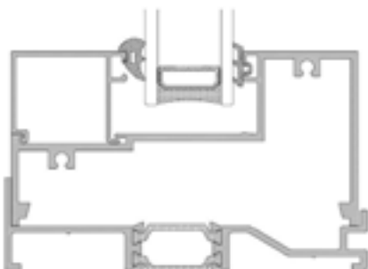
Cill Detail
