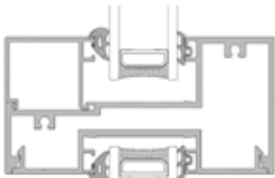
Transom Detail
