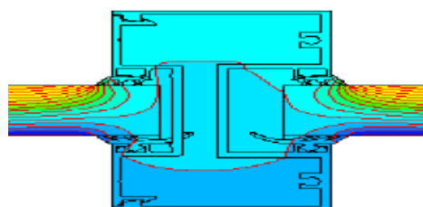
Mullion Detail
