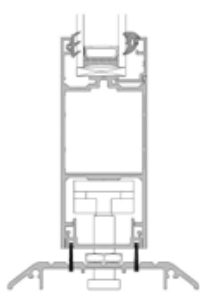
Threshold Detail
