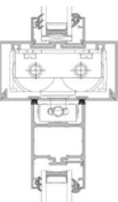
Transom Detail
